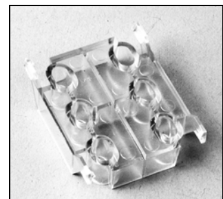
Spacer Block 2" LP Support Bracket PCN 5003156000
