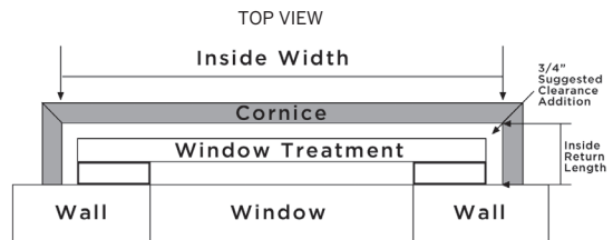
Outside Mount (top view)
