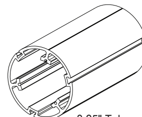
3.25" Tube
