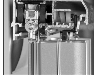
End View - Installation Complete
